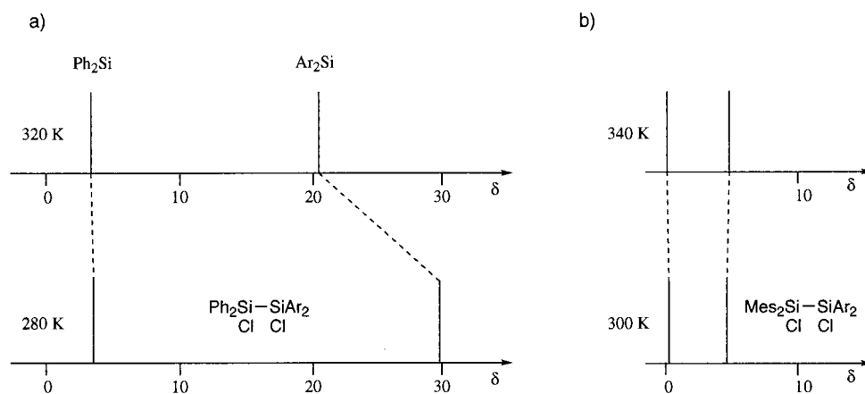
Fig. 1. ^{29}\text{Si} -NMR spectra of 10b and 33b at variable temperature; \text{Ar} = 2-(\text{Me}_2\text{NCH}_2)\text{C}_6\text{H}_4 ; (a) Spectra of 10b at 320 K (top) and 280 K (bottom); (b) Spectra of 33b at 340 K (top) and 300 K (bottom).
