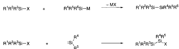
Scheme 1. Formation of Si–Si bond; M = Li, Na, MgHal; X = H, Hal.
